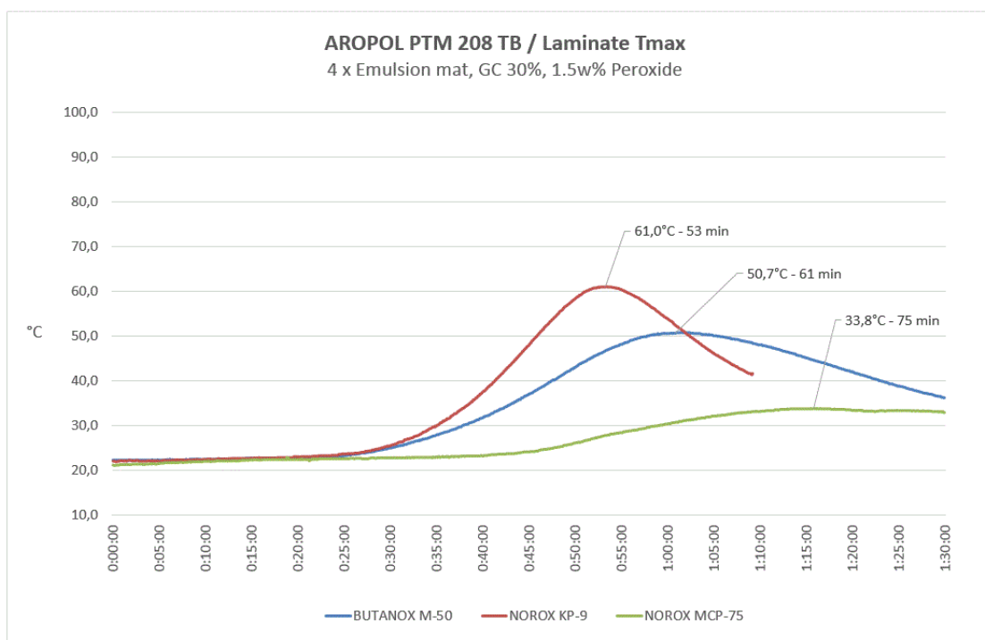
Laminate exotherm with various peroxides.
